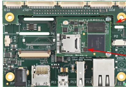
TM1 module with 1GHz ARM Cortex A9 processor, memory, Flash, Wifi and Bluetooth
